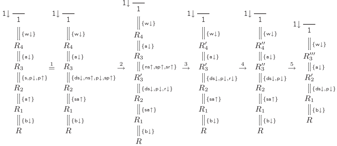
Fig. 6 Cut elimination for \text{SELSU} \cup \{1\downarrow\}
